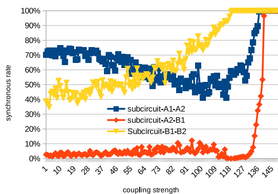
Figure 2. Synchronous rate of Circuit-A and Circuit-B.
