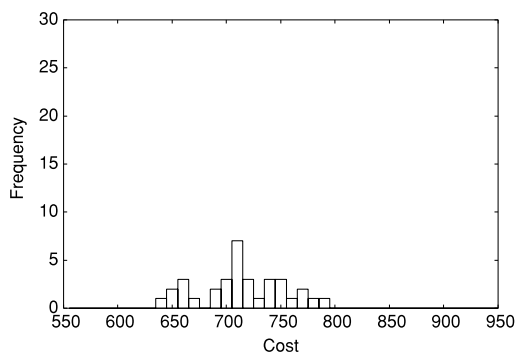
Fig. 8 Frequency distribution of solutions with fully developed chaos noise for Nug12.
