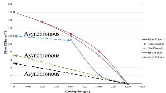
Fig. 8. Relationship between coupling strength and phase difference.
