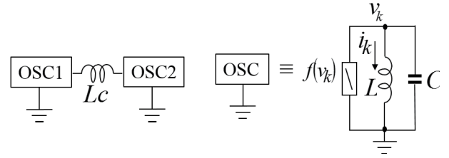
Figure 1: Circuit model.
