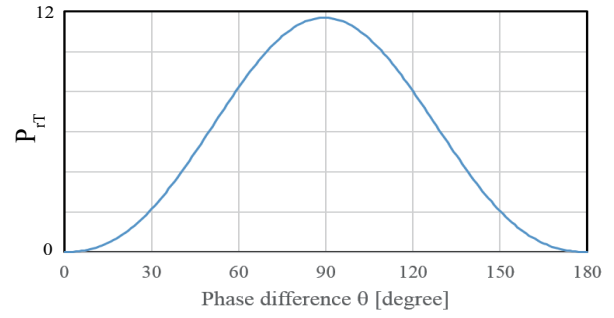
Figure 7: Theoretical results of P_{rT}(\alpha = 0.05 and \epsilon = 0.10) .
