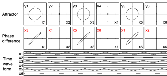
Figure 7: Synchronization results for N = 6 (at \alpha=0.64 ).
